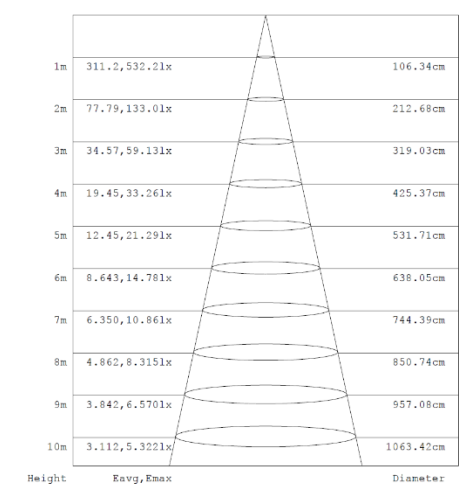
Diagram for RULFX-01 in 6W, 4000K Other diagrams available on request
