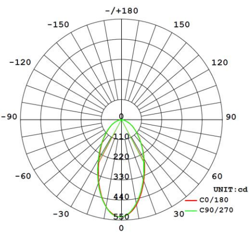
Diagram for RULFX-01 in 6W, 4000K Other diagrams available on request
